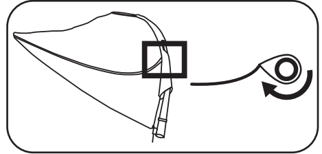
Figure 4: Downhaul slowly until the front of the foot batten "pops" to the side of the mast.
