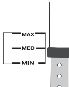
Fig. 1: Downhaul until the calibration mark lines up with the bottom of the mast.
