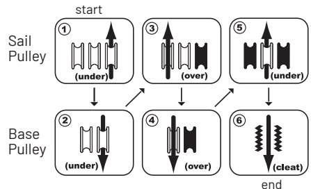
Fig. 12: Threading the tack pulley for a Chinook-style extension.
